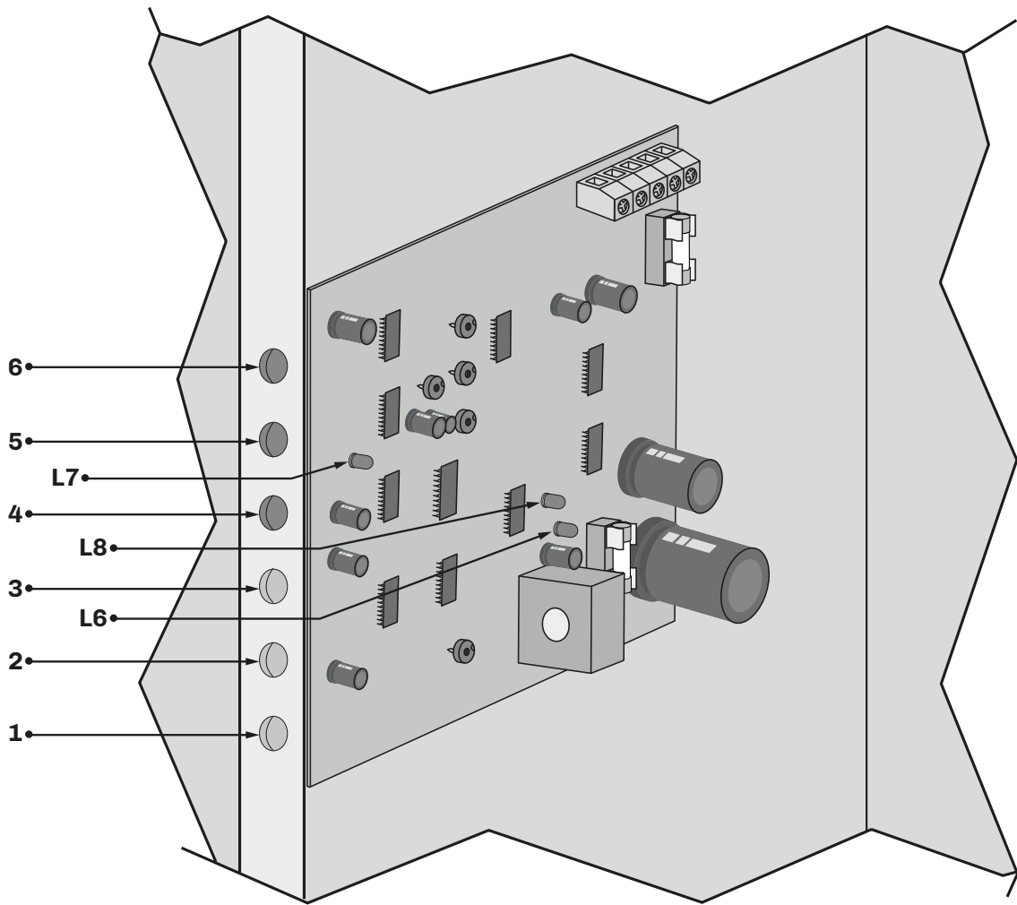
Fig. 24. Interface LED
